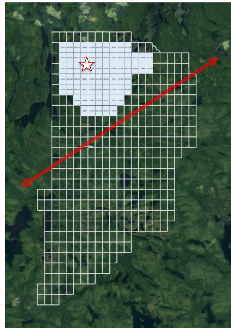
Satellite image showing obvious deformity around the Renzy mine. The red line shows the Renzy Shear Zone which could be an important factor in nickel magma emplacement.
